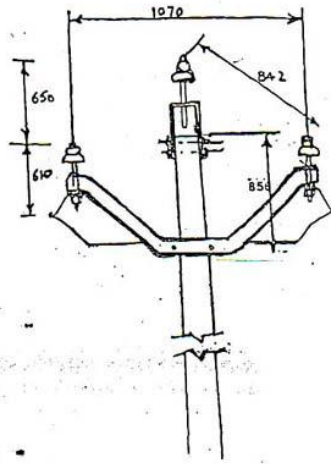
11KV IN DELTA FORMATION
