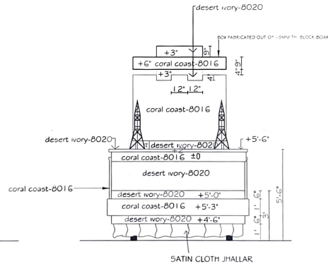
REAR ELEVATION
