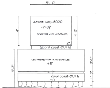
REAR ELEVATION
