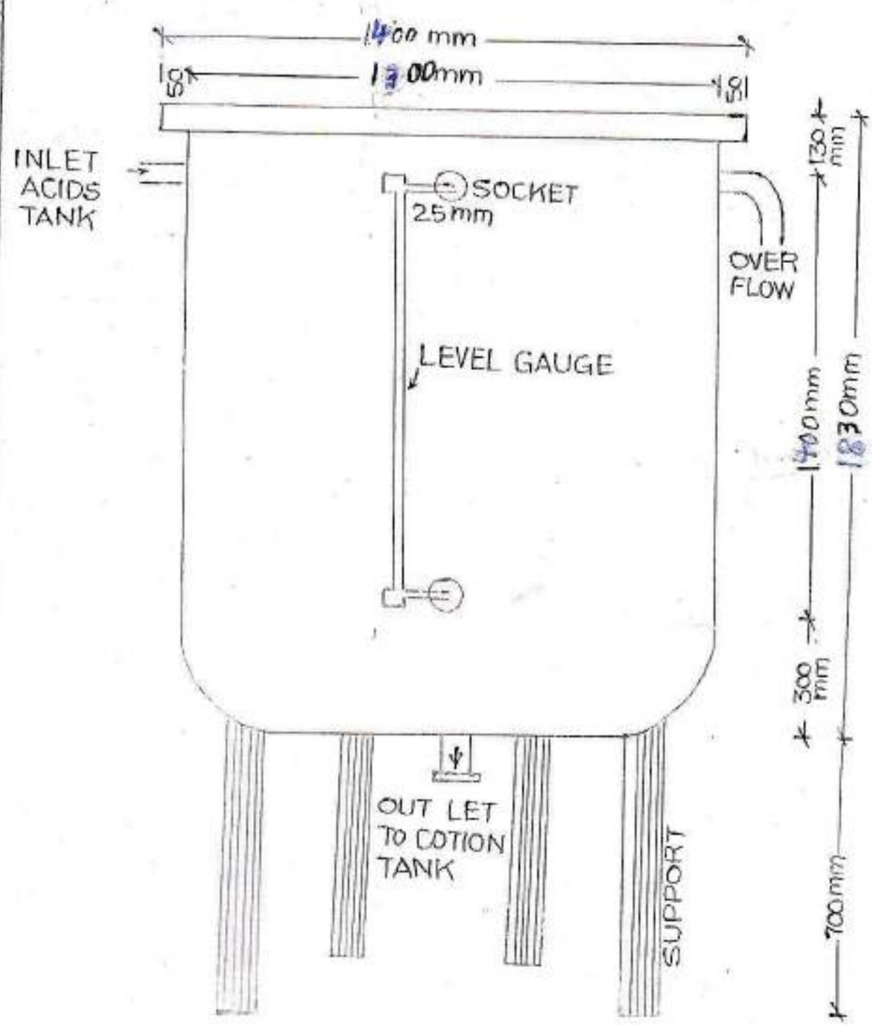
INJECTION TANK (FOR REGENERATION OF CATION TANK)
